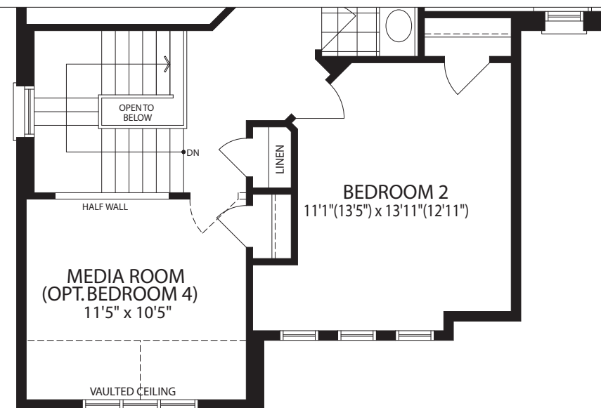
PART. SECOND FLOOR ELEVATION 'B'
