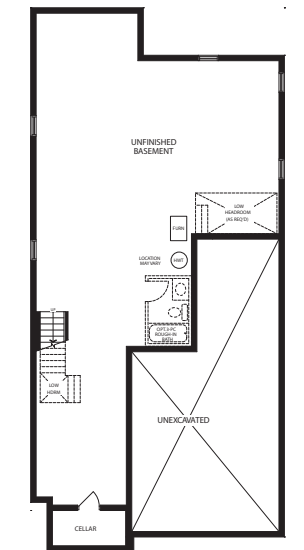
OPT. BASEMENT W/TANDEM GARAGE ELEVATION 'A'
