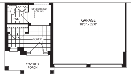
PART. GROUND FLOOR ELEVATION 'B'
