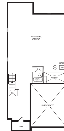
BASEMENT ELEVATION 'A'
