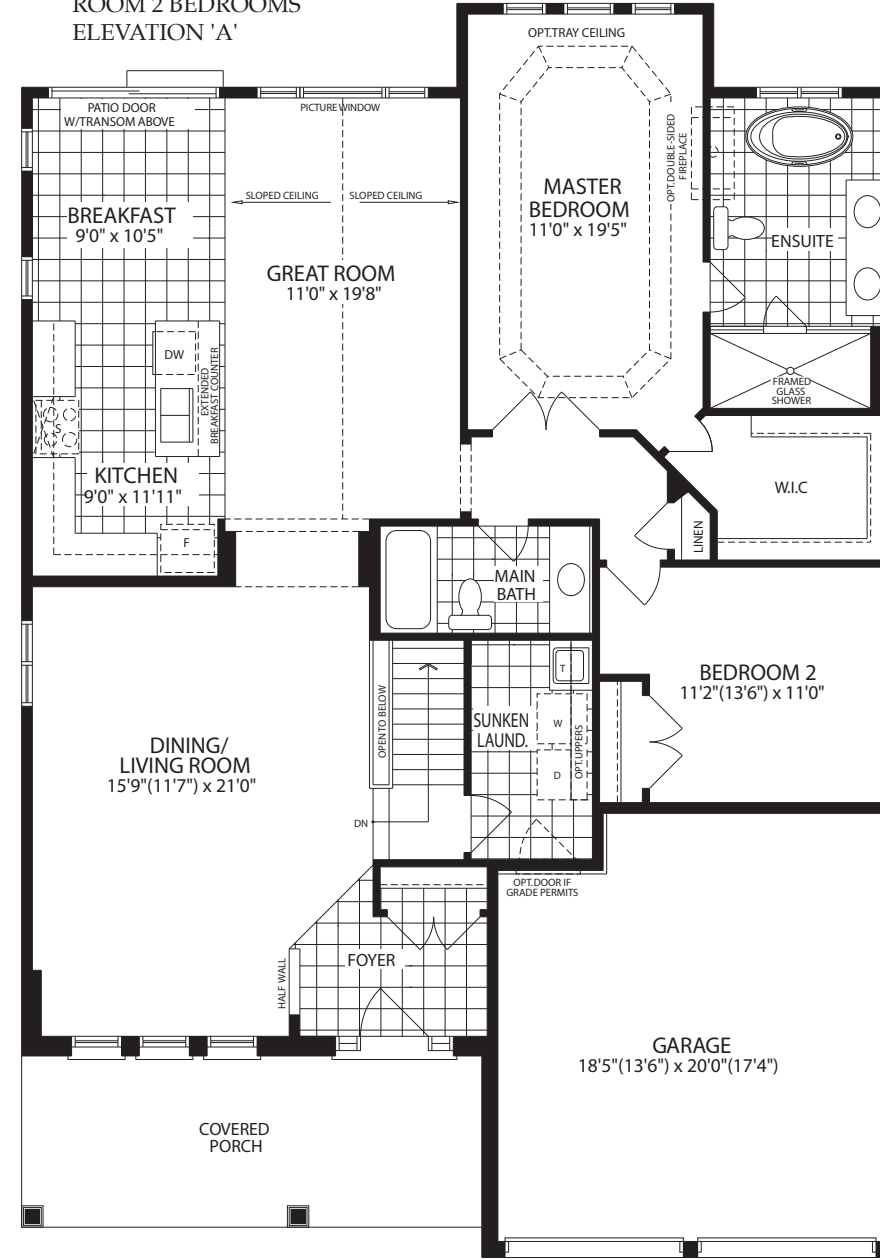
OPT. GROUND FLOOR 2 BEDROOMS ELEVATION 'A'
