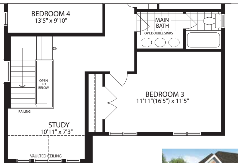
PART. SECOND FLOOR ELEVATION 'B'
