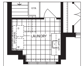
PART. OPT. SECOND FLOOR ELEVATION 'A'
