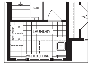
PART. OPT. SECOND FLOOR ELEVATION 'B'
