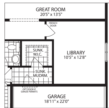
PART. OPT. GROUND FLOOR MUDROOM FOR OPT. SECOND FLOOR
