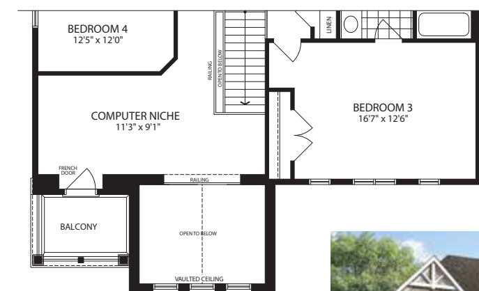
PART. SECOND FLOOR ELEVATION 'B'
