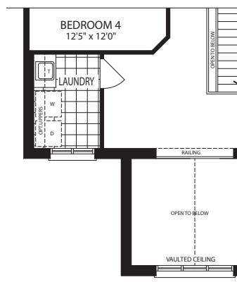
PART. OPT. SECOND FLOOR LAUNDRY ELEVATION 'A'
