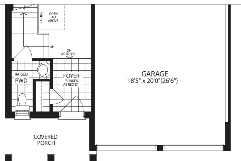
PART. GROUND FLOOR ELEVATION 'B'
