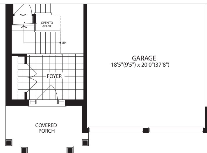
PART. GROUND FLOOR W/OPT. TANDEM GARAGE ELEVATION 'B'
