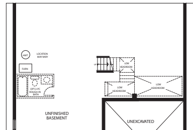
PART. BASEMENT W/OPT. GROUND FLOOR STUDY ELEVATION 'A' (ELEVATION 'B' SIMILAR)
