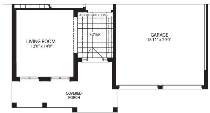
PART. OPT. GROUND FLOOR W/STUDY ELEVATION 'B'
