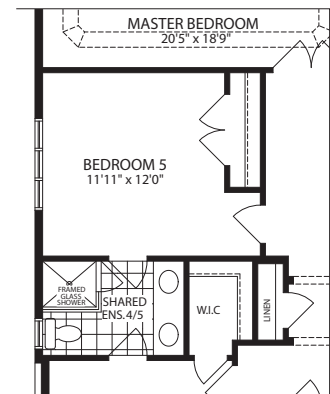
PART. OPT. SECOND FLOOR W/5 BEDROOMS ELEVATION 'A' (ELEVATION 'B' SIMILAR)
