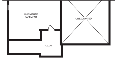
PART. BASEMENT ELEVATION 'B'
